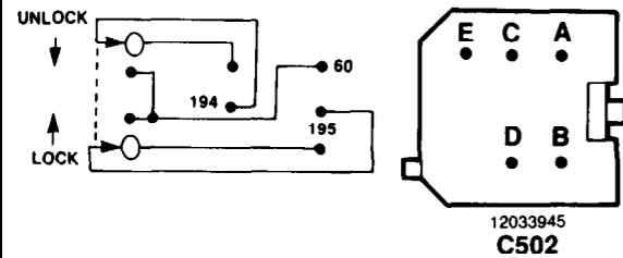
LH POWER DOOR LOCK SWITCH
